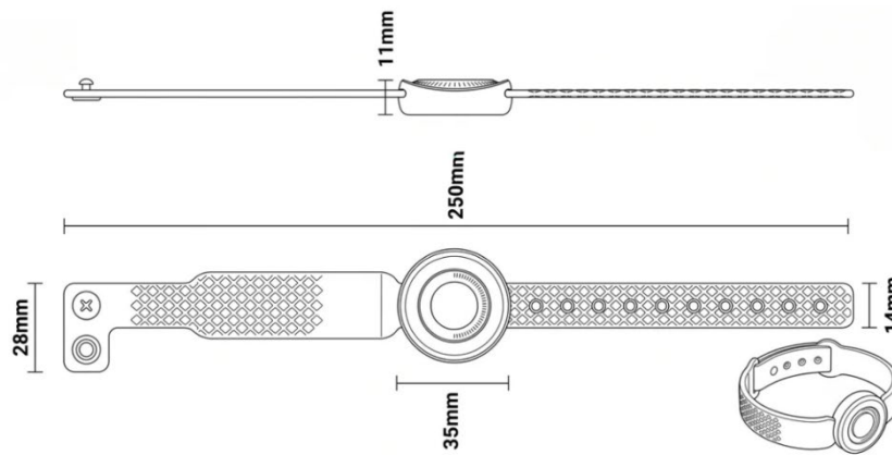
PINIX TOB-1 Tag Mechanical Drawings
